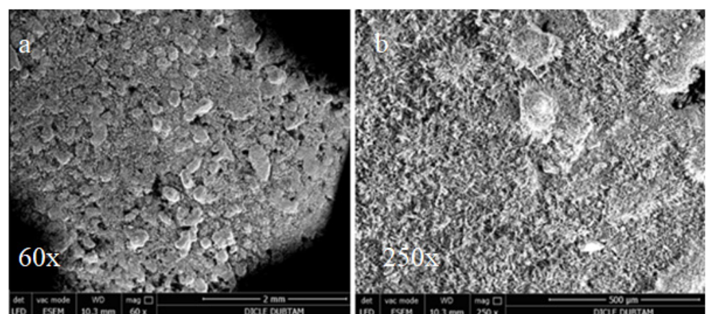
Figure 12. SEM images of SFS replacement bar samples cured 90 days in hydropath: (a) 60 \times (b) 250 \times .
