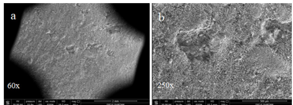
Figure 11. SEM images of control bar samples without replacement cured for 90 days in hydropath: (a) 60 \times ; (b) 250 \times .
