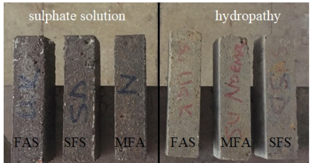
Figure 10. Plain concrete (MFA), silica fume (SFS) and fly ash (FAS) mineral additives substituted bar samples with curing conditions in hydropath and sulphate solution.
