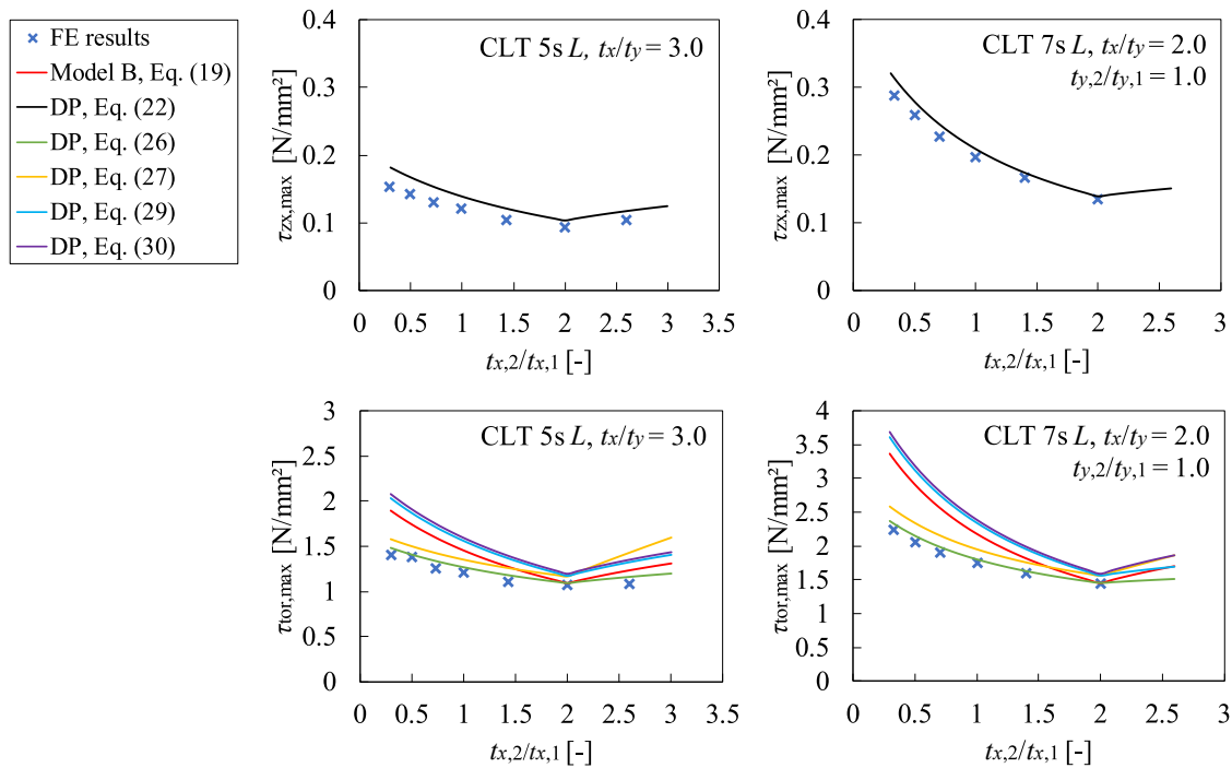
Fig. 8. Comparison between FE results and model predictions for design relevant stresses for varying lay-ups 0.31 \leq t_{x,2}/t_{x,1} \leq 2.6 of CLT 5s and 0.33 \leq t_{x,2}/t_{x,1} \leq 2.0 of CLT 7s.
