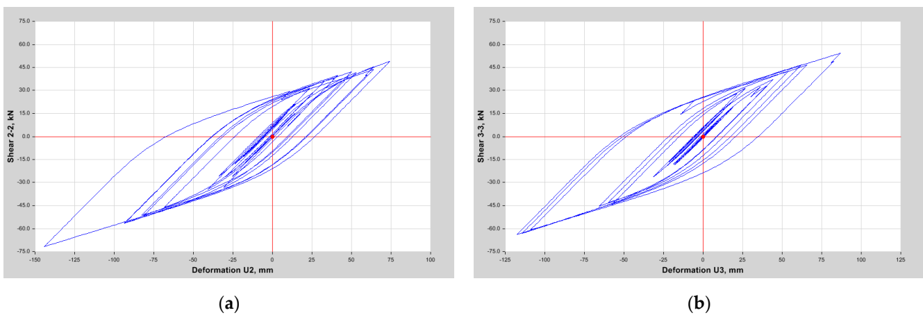
Figure 13. HDRB's hysteresis area (data from Dar El Beida seismic record): (a) in the X direction; (b) in the Y direction.
