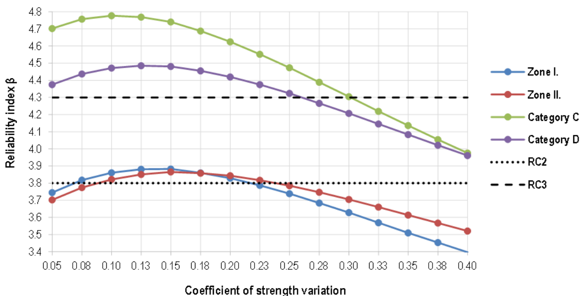
Figure 3 Reliability index \beta as a function of coefficient of strength variation
