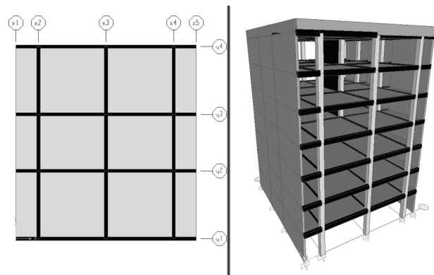
Figure 15 3D structure model in SAP2000
