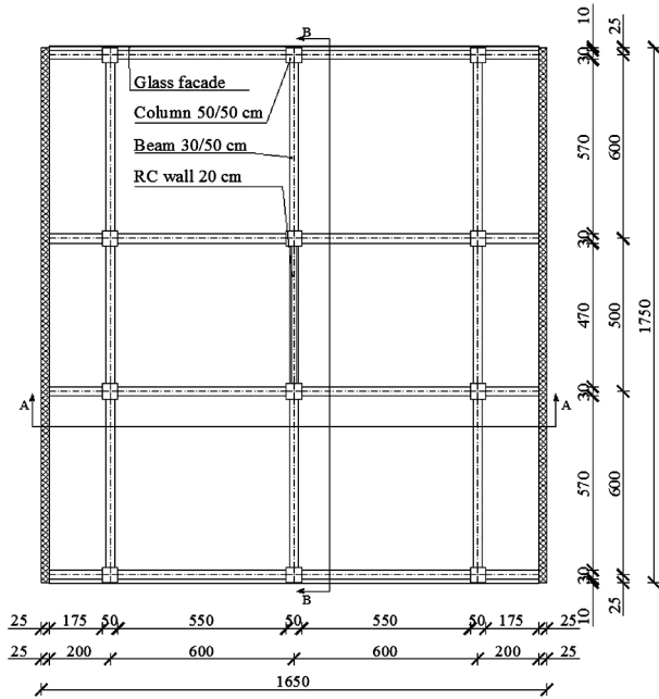
Figure 12 Plan of the building
