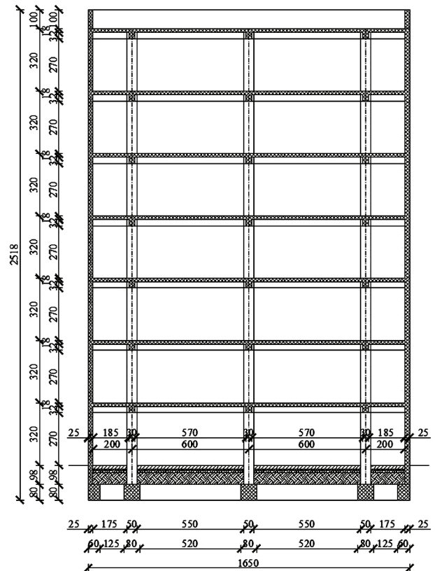
Figure 14 Cross-section A-B
