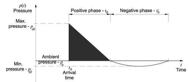
Figure 2 Pressure-time profile of the explosion wave
