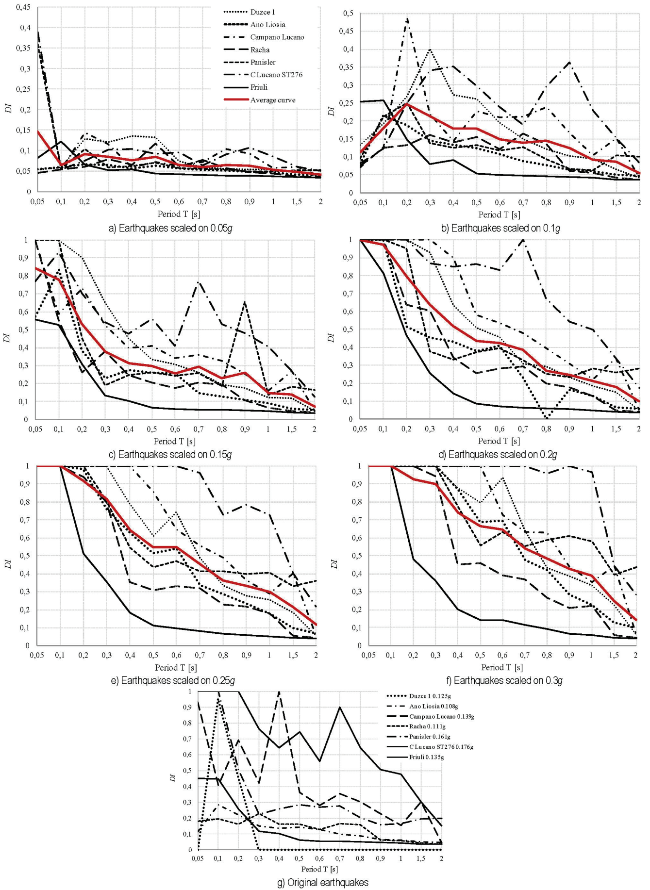
Figure 4 Spectral damage functions for URM with flexible floors defined by the following parameters BS_{\gamma}=0.1WK_{\gamma}=0K_{\alpha}\zeta=5\% and a) earthquakes: scaled on 0.05g, b) Earthquakes scaled on 0.1g, c) Earthquakes scaled on 0.15g, d) Earthquakes scaled on 0.2g, e) Earthquakes scaled on 0.25g, f) Earthquakes scaled on 0.3g, g) Original earthquakes
