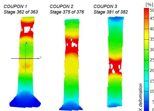
Figure 12 Elongation and corresponding change in cross-sectional width and thickness during fracture (GOM ARAMIS)
