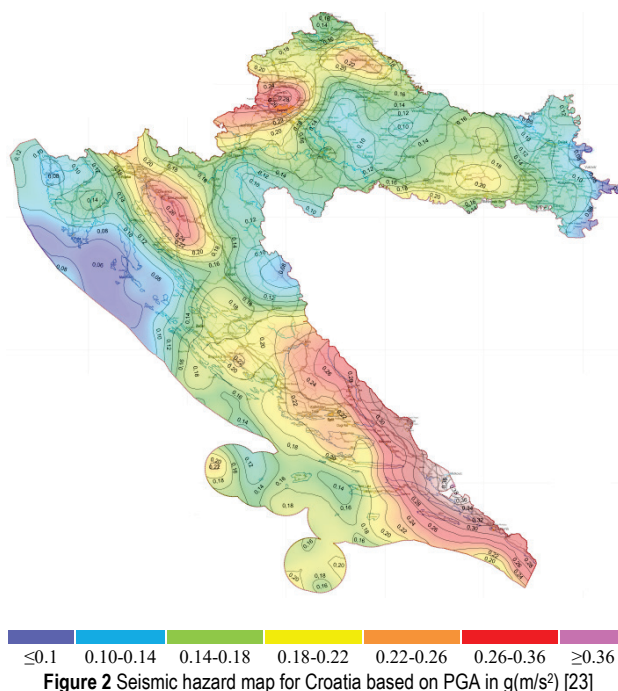
Figure 2 Seismic hazard map for Croatia based on PGA in g/(m/s²) [23]
