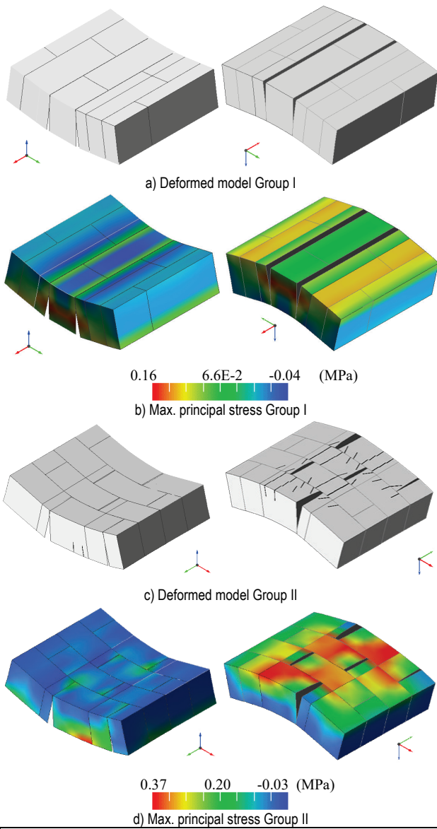
Figure 8 Numerical test results at F_{max}
