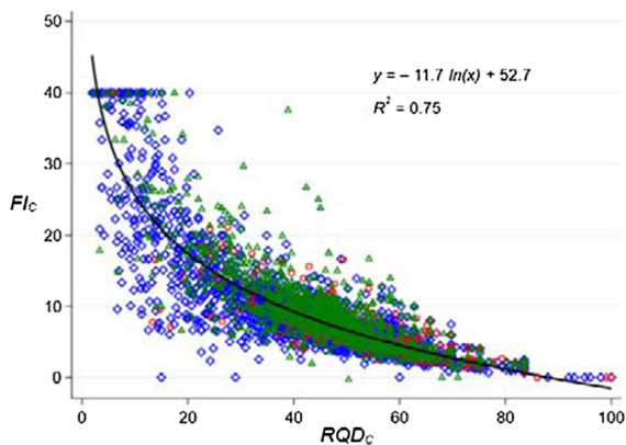
Fig. 11 Correlation plot of FI_C versus RQD_C
