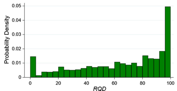
Fig. 6 Probability density histogram of RQD
