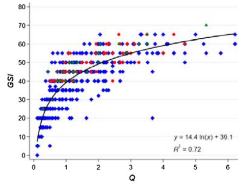
(b) Correlation plot of GSI versus Q
