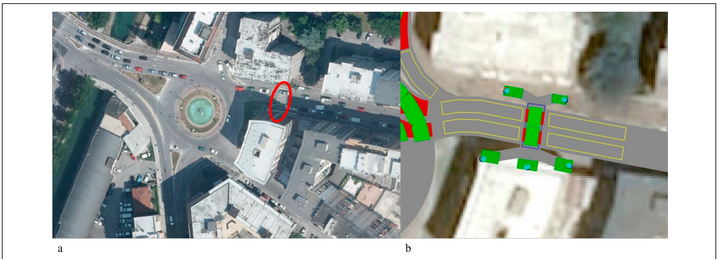
Figure 2 Study location: (a) urban roundabout set in Monfalcone (GO) Italy; (b) the crosswalk under study modelled in Vissim/Viswalk
