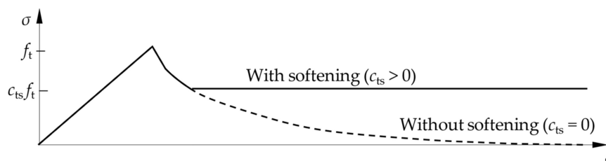
Figure 8. Tension stiffening.
