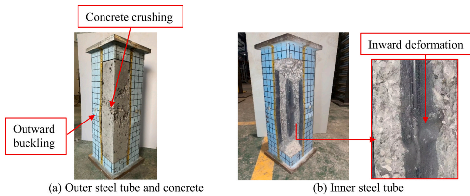
Fig. 9. Failure modes of tube and concrete of a typical specimen.
