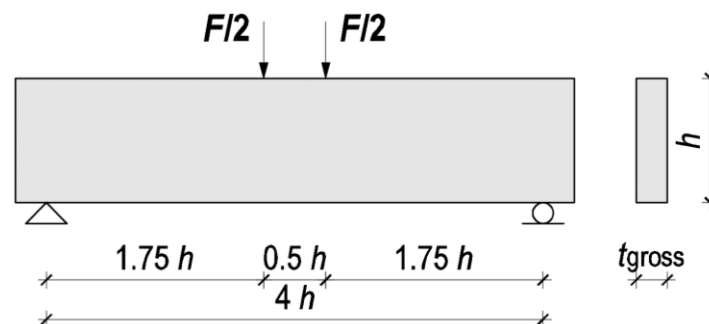
Figure 5 Geometrical properties of analyzed CLT beams
