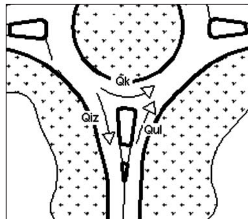
Slika 1 Veličine prometnog opterećenja na ulivu, izlivu i u kružnom toku Figure 1 Traffic flow rates entry flow, exit flow and circulating flow
