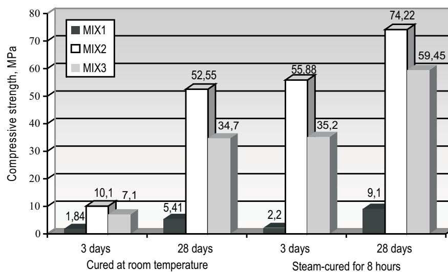
Figure 2 Relationship between compressive strength and curing time of the geopolymer concrete (MIX1, MIX2 and MIX3).
