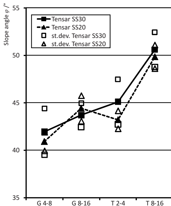
Figure 9 Mean values of slope angles for geogrids Tensor SS30 and Tensor SS20 in natural gravel G 4-8, G 8-16 and crushed gravel T 2-4 and T8-16 with mean standard deviation of tests on both grids.
