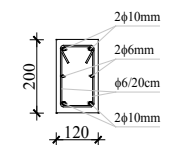
Figure 2 Geometric and reinforcement details of the model specimens
