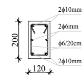
Figure 2 Geometric and reinforcement details of the model specimens
