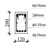
Figure 2 Geometric and reinforcement details of the model specimens
