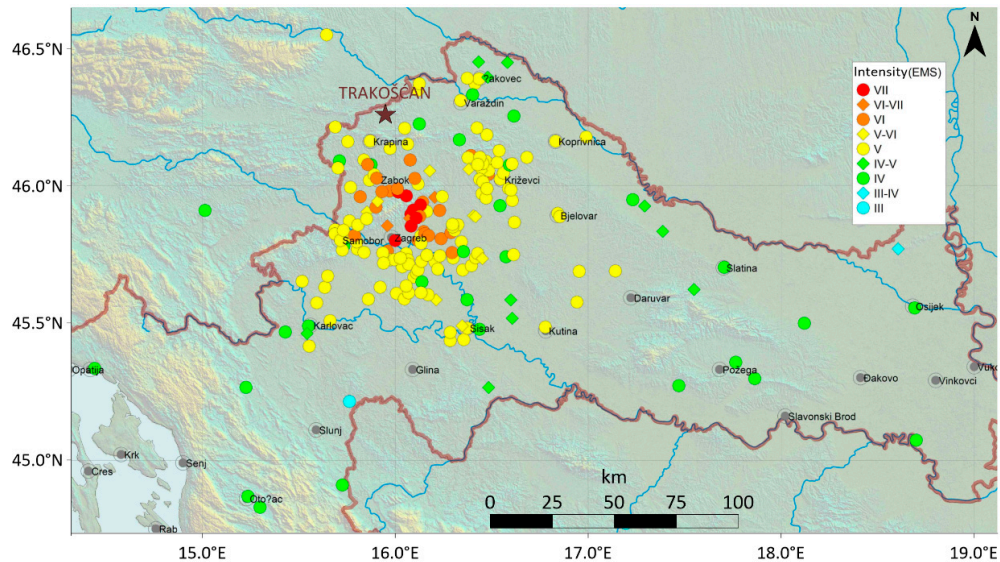
Figure 3. Adapted preliminary intensity map of Zagreb M5.5 2020 earthquake, prepared by the Seismological Survey, Department of Geophysics, Faculty of Science, Zagreb, Croatia [19]. The position of Trakošćan Castle is marked with a brown star.
