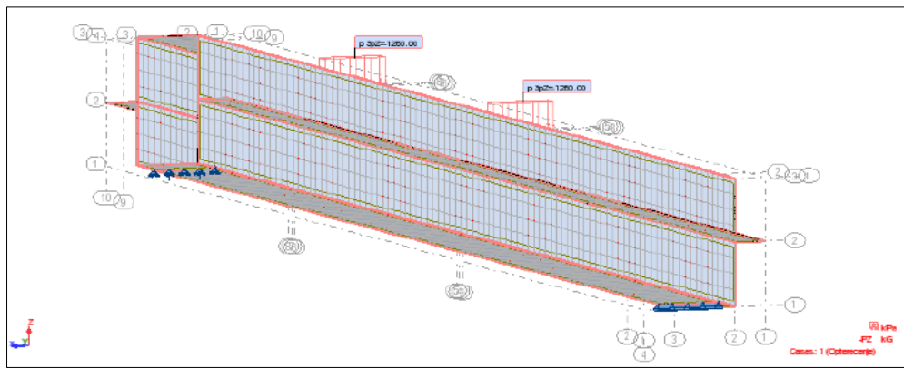
Figure 12. Mesh of finite elements and loads
