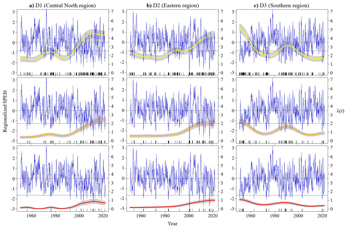
Figure 8. Regionalized SPEI6 from 1950 to 2022. Time-dependent occurrence rates of drought periods in homogeneous regions (a) D1, (b) D2, and (c) D3, as shown in Figure 4a–c, respectively. Left y-axis: the regionalized SPEI6 in dark blue. Right y-axis: the number of months under drought conditions per year, \lambda(t) , categorized as moderate (in yellow), severe (in orange), and extreme (in red); the confidence band is represented by the grey area around \lambda(t) . Horizontal dashed lines, distinct from zero, indicate the thresholds (DT) adopted for different types of drought conditions. Vertical ticks mark the dates of periods under drought conditions.
