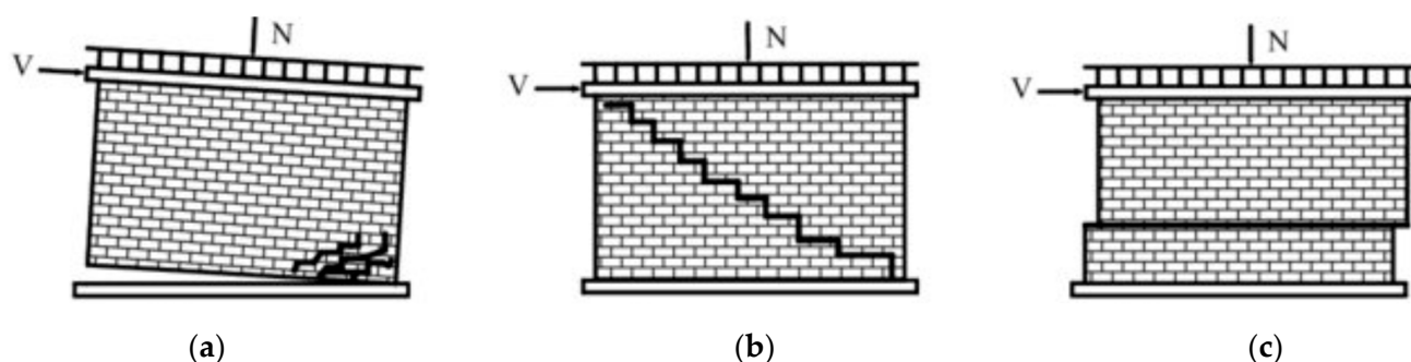
Figure 6. Crack patterns in UnReinforced Masonry (URM) walls: (a) rocking failure; (b) diagonal cracking; (c) bed-joint sliding [7].
