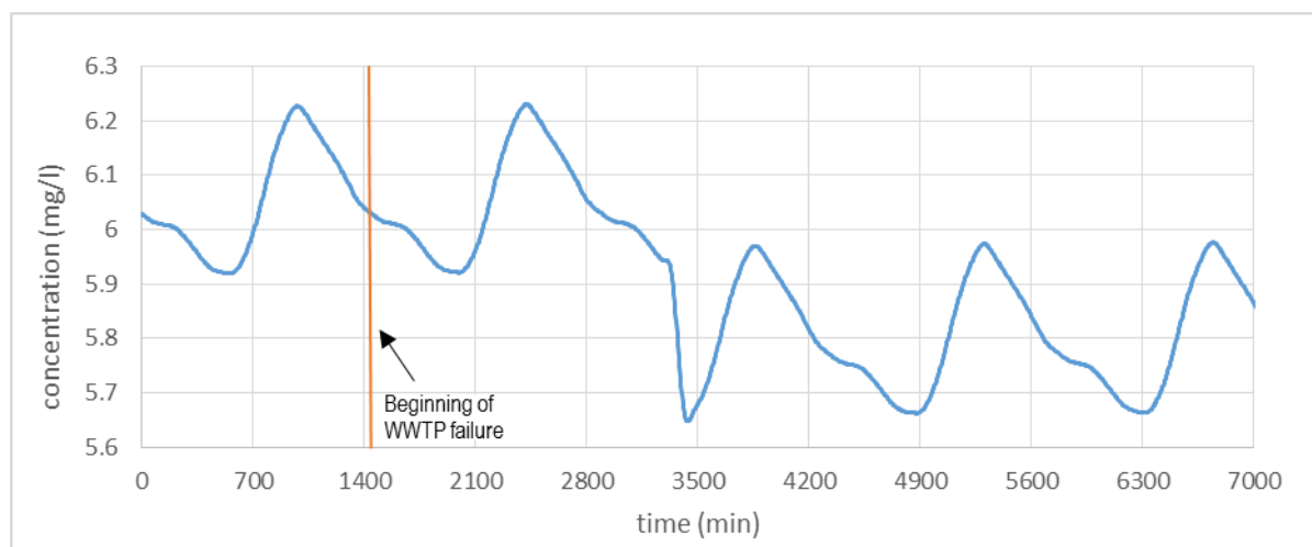
Figure 5 Change in dissolved oxygen concentration at 00 + 543 rkm in the period between January 14, 2015 (11:59 p.m.) and January 19, 2015 (11:59 p.m.)
