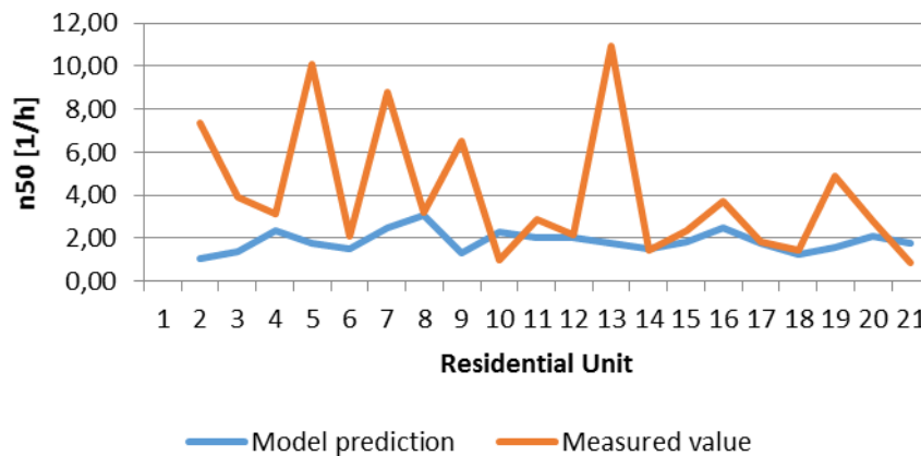
Figure 3 Results of airtightness prediction model from Sweden [6]
