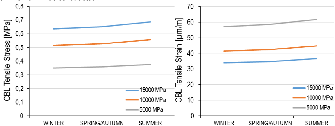
Figure 8 Correlation of stress and strain at the bottom of CBL with respect to its modulus of elasticity value
