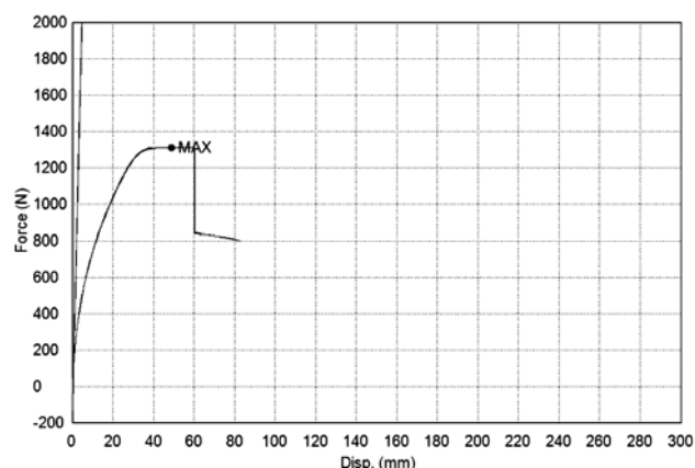
Figure 10 Breaking of a single strap sample
