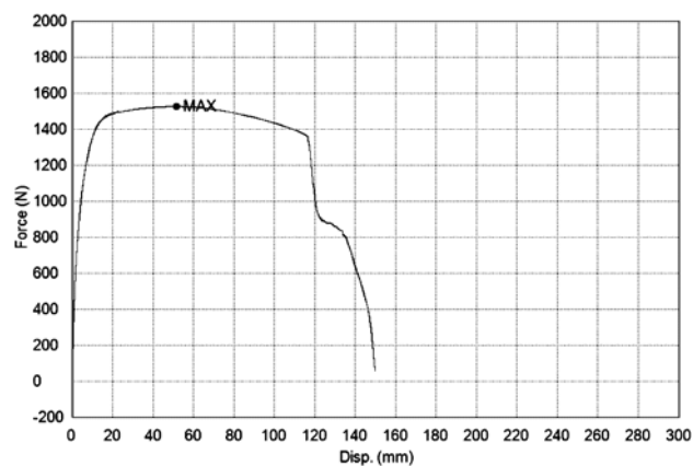
Slika 11 Breaking of a six strap sample
