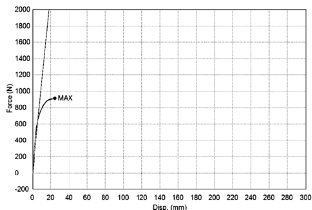
Slika 9 Breaking of a triple strap sample
