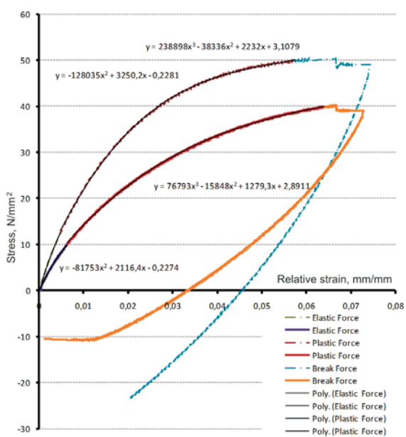
Figure 14 Idealised stress/strain diagram with a quadratic and a cubic curve
