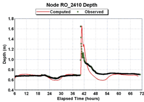
Metering station 1
