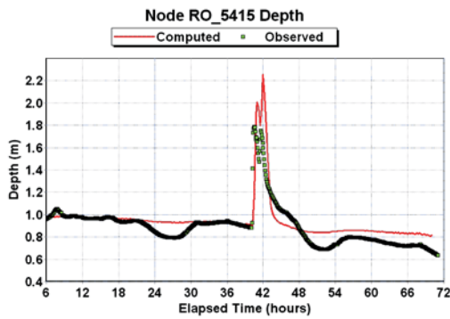
Metering station 5
