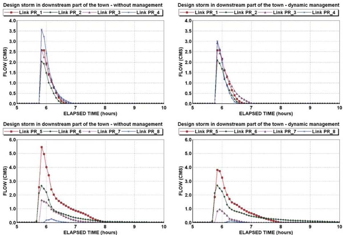
Figure 11 Flow rate ( m^3/s ) at stormwater overflows for design storm in downstream (eastern) part of the town - without and with dynamic management Slika 11. Protok na preljevim ( m^3/s ) za projektni pljusak u nizvodnom (istočnom) dijelu grada - bez upravljanja i s dinamičkim upravljanjem
