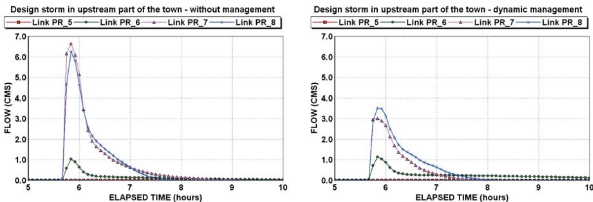
Figure 12 Flow rate ( m^3/s ) at stormwater overflows for design storm in upstream (western) part of the town - without management and with dynamic management Slika 12. Protok na preljevim ( m^3/s ) za projektni pljusak u uzvodnom (zapadnom) dijelu grada - bez upravljanja i s dinamičkim upravljanjem
