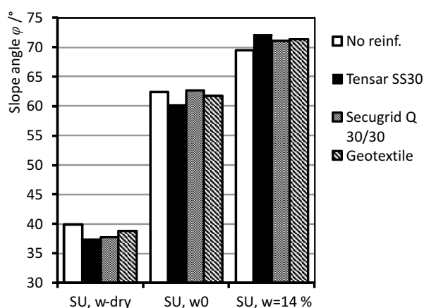
Figure 10 Slope angle \phi for dry sand, sand with natural moisture content and 14 % moisture content
