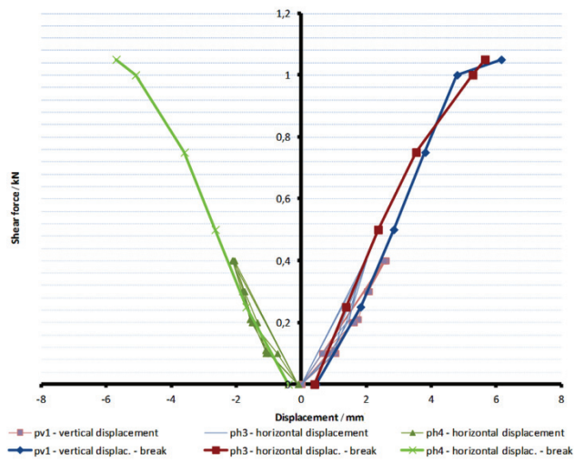
Figure 9 Force/displacement diagram
