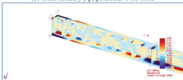
c) Normal stresses z-z perpendicular to the fibres
