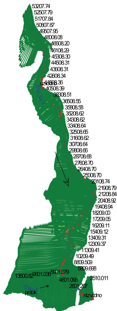
Figure 3 Geometry of the River Danube prepared for modeling ( HEC-RAS)
