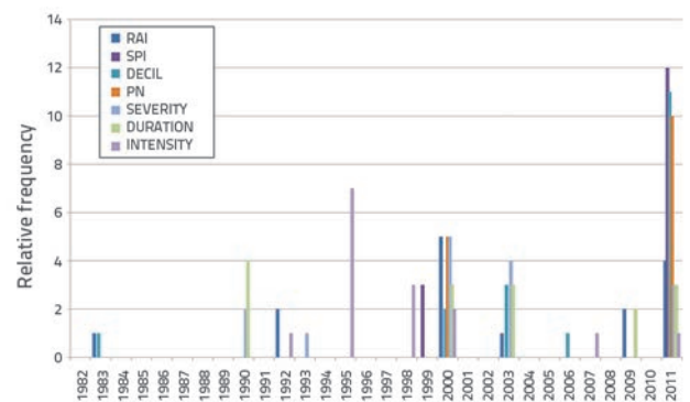
Figure 9. Frequency of driest years according to individual methods
